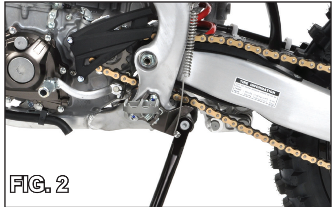
5204-00 Kickstand Installed
